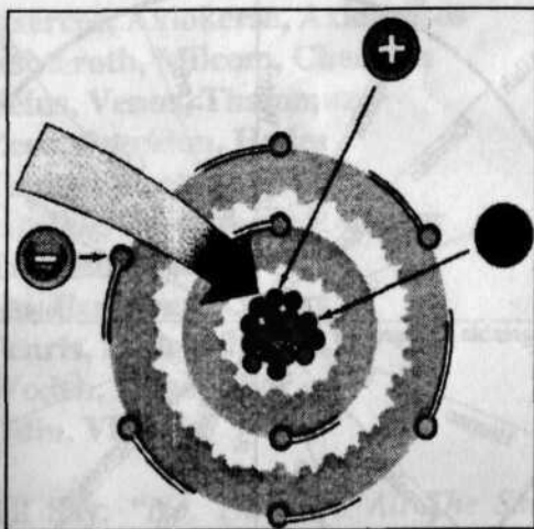
The Atom Consisting Of Positively Charged Nucleus Sur- rounded By A System Of Electrons.
